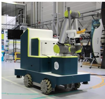
Cobotics – MASCOT Project
