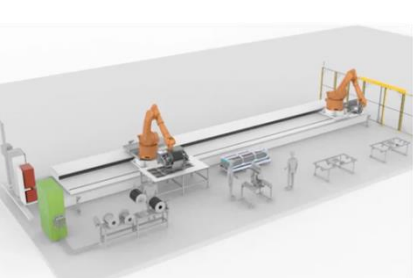
Automated NCF+UD lay-up & forming (Q3 2019)
