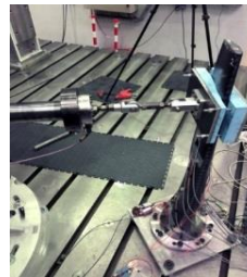
QRS sensors inserted – response under loading, 2018
