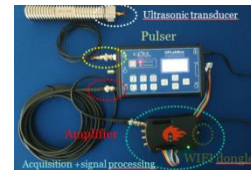
Embedded US for loss of tightening in a bolt, 2018
